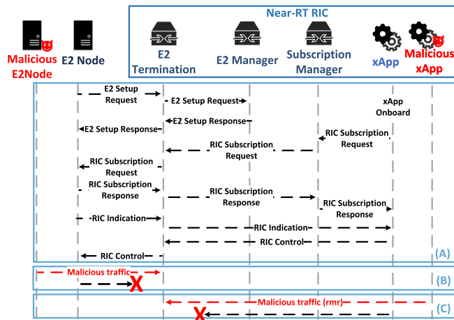
FIGURE 2. The E2 communication process between xApp and E2 node, and the possible attack scenarios involved.
