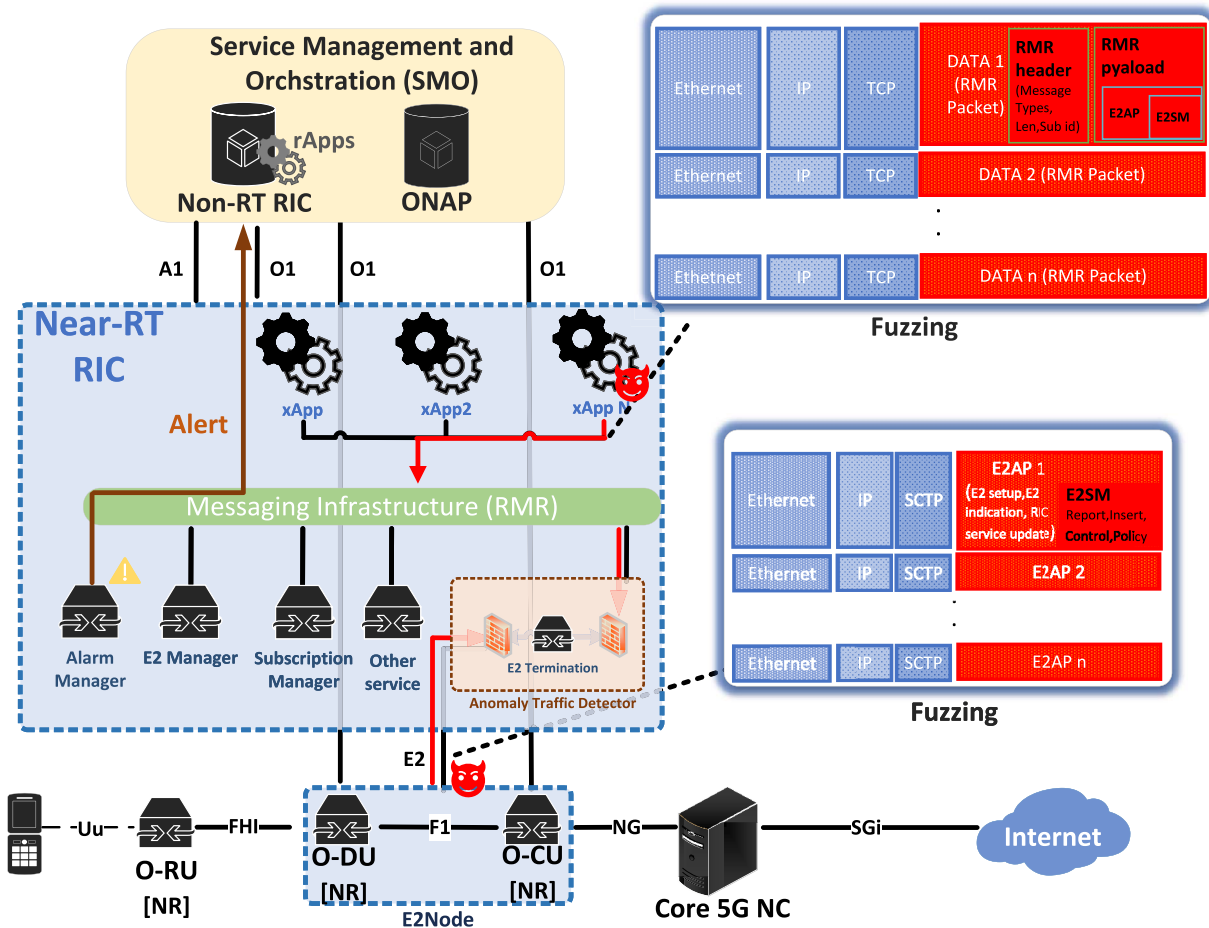
FIGURE 1. Overview of O-RAN architecture with anomaly traffic detector framework.
