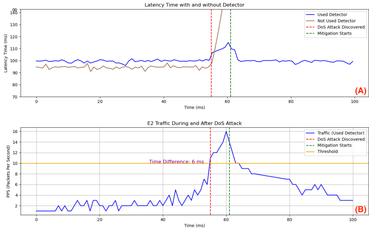
FIGURE 5. Latency time with and without detector & E2 traffic during and After DoS attack.
