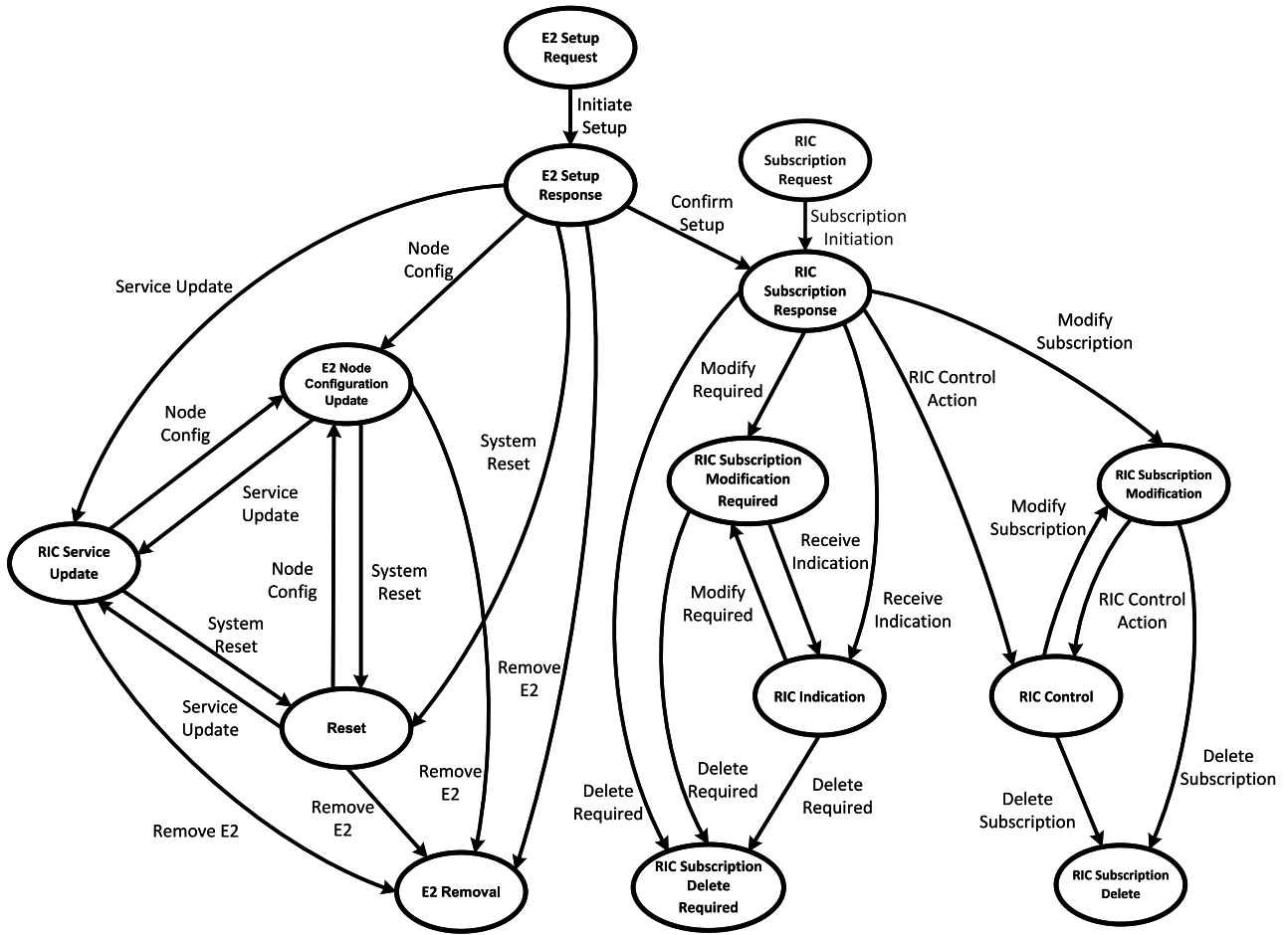
FIGURE 4. The state machine analysis module.
