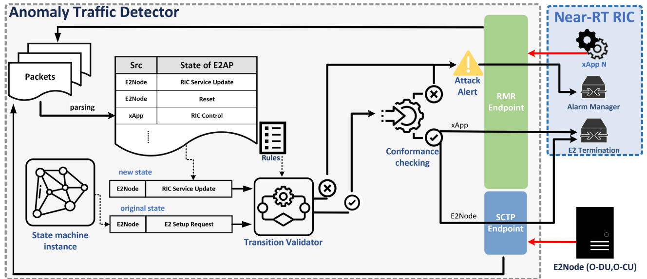
FIGURE 3. Anomaly traffic detector architecture.
