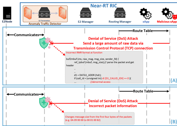
FIGURE 6. Mitigation of malicious xApp non-compliant packet attacks using anomaly traffic detector.
