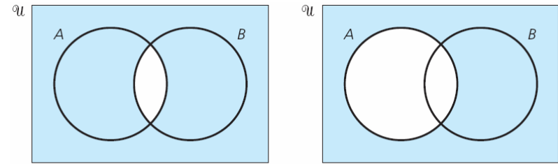
(a) \overline{A \cap B} (b) \bar{A}
