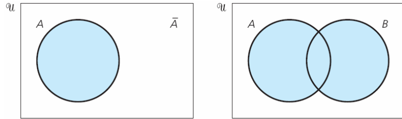
(a) (b) A \cup B
