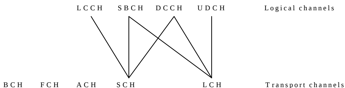
Figure 4: Mapping from logical to transport channels in downlink.
