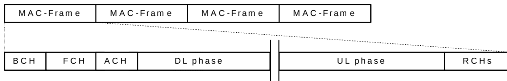
Figure 3: Basic MAC frame structure
