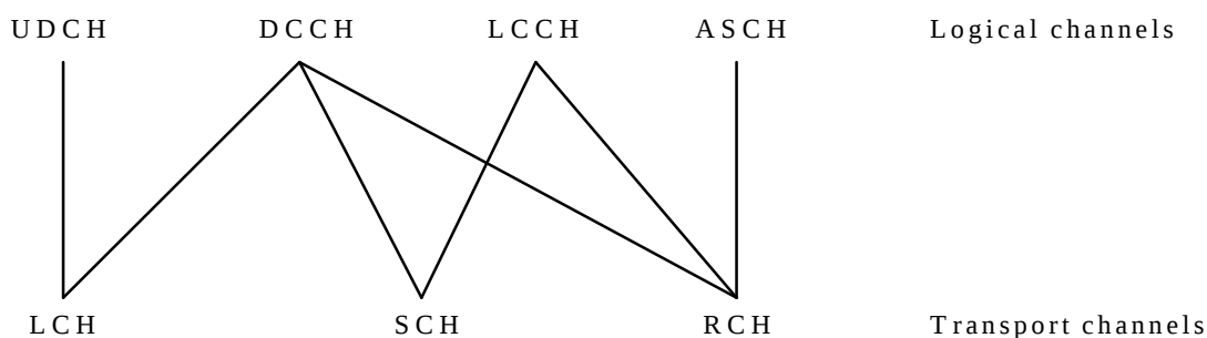
Figure 5: Mapping from logical to transport channels in uplink.
